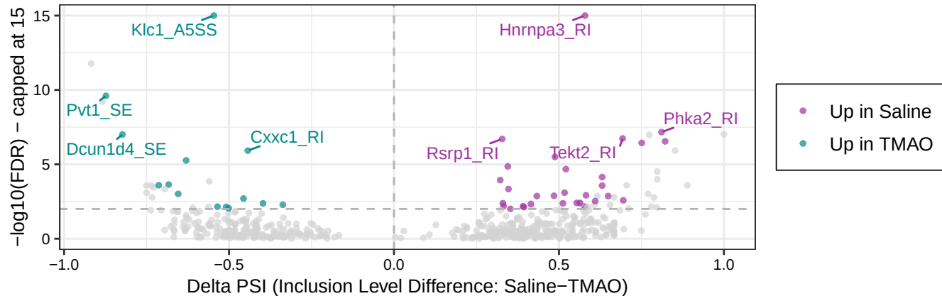
Volcano Plot for Differential Splicing Analysis
